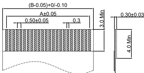
适用扁平线 (Applicable Flat Cable)
