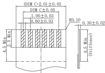
RECOMMENDED FFC/FPC
