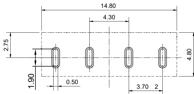
TOP VIEW P.C.B. LAYOUT
